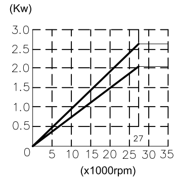
Power-diagram
