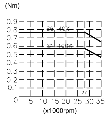
Torque-diagram
